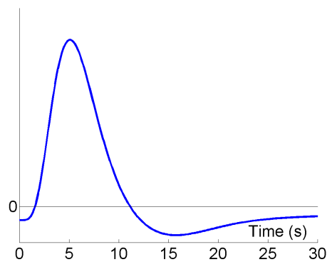
HRF
