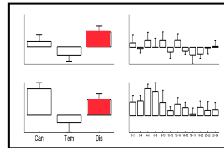
+ Dispersion
