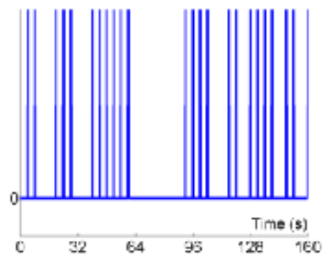
Stimulus ("Neural")
