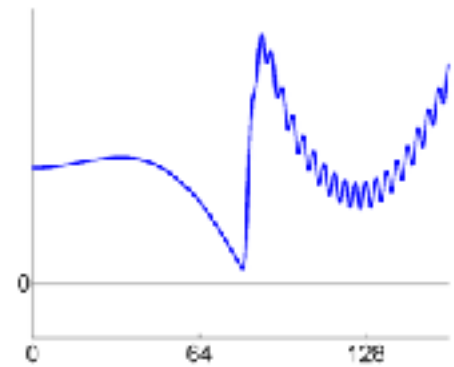
Predicted Data
