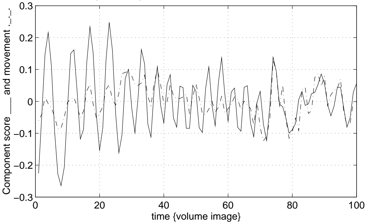
Eigenimage 6 – 1.6 percent of variance
