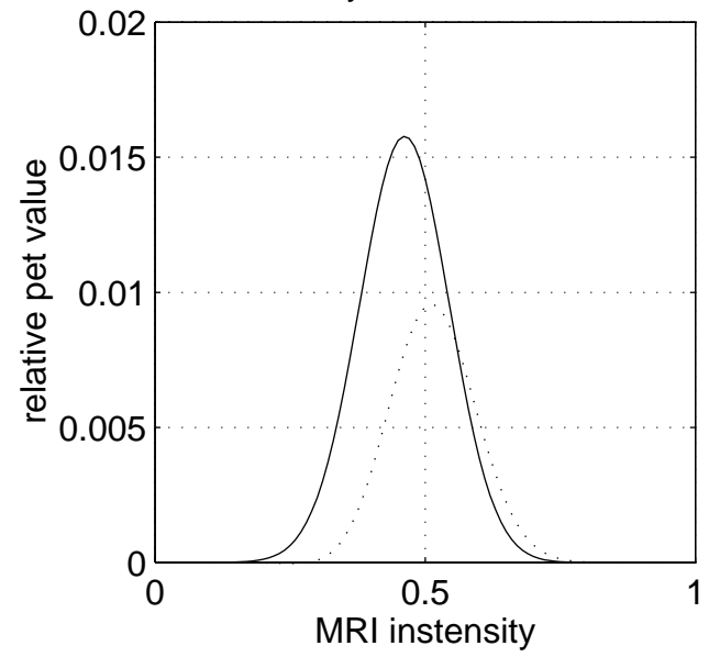
intensity transformations
