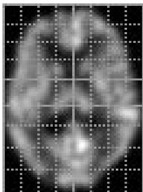
transformed & convolved
