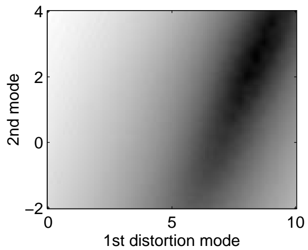
Error surface
