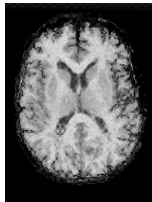
coregistration
