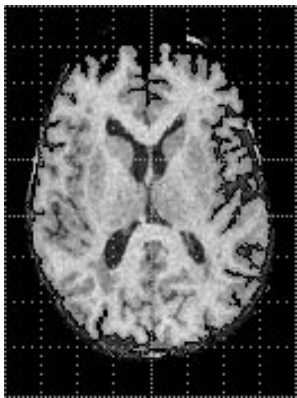
spatially transformed
