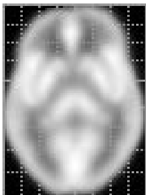
least squares
