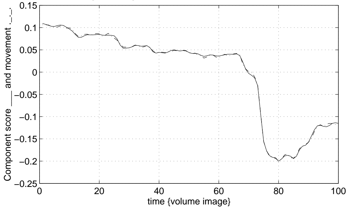
Eigenimage 1 – 57.2 percent of variance
