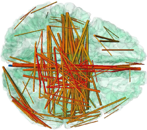
Fig. 3. A connectivity map, identifying significantly-connected regions via cylinders of differing width.
